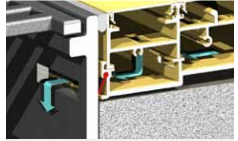
Sill drainage a speciality. Contact AWS Tech Support for varying options.
