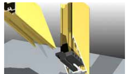
Elevate™ Commercial awning and casement sashes are fabricated with heavy duty nylon corner stakes. These keep the joints tight and waterproof.
