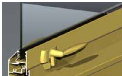
As the MIRO™ lever is operated the nylon retention folds up and allows the sash to swing open.
